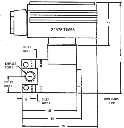
Dimensional Diagram of 24476 Timer and 20311-3 Sol. Valve (Sold Separately)
